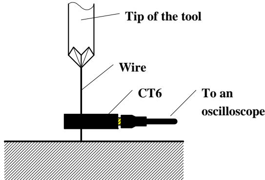
Figure 4. Current Measurement Setup in the Tool
