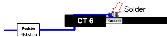
Figure 9. Measurement of possible current exposure on direct contact with CT6 probe
