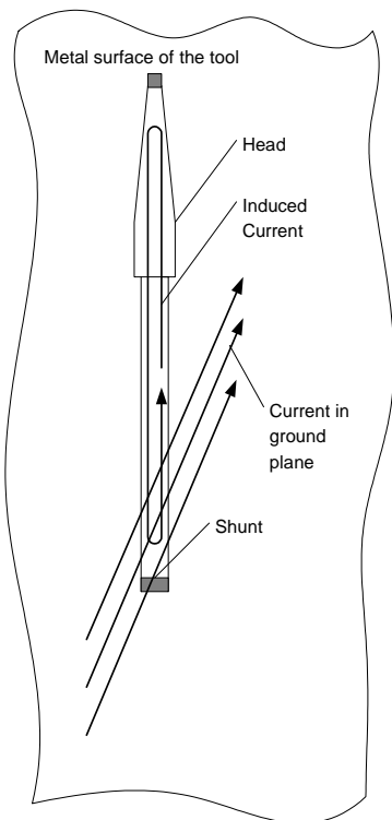
Figure 6. Inductive Coupling Between Ground Current and the Head
