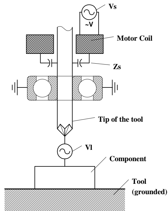
Figure 2. Generation of Voltage in a Tool via Capacitive
