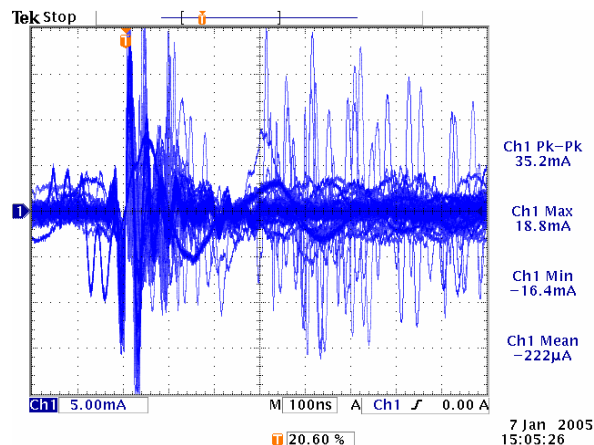
Figure 7. Current induced by transformer coupling in the tool (peak value – 35mA). Multiple signals are often present on ground as seen.
