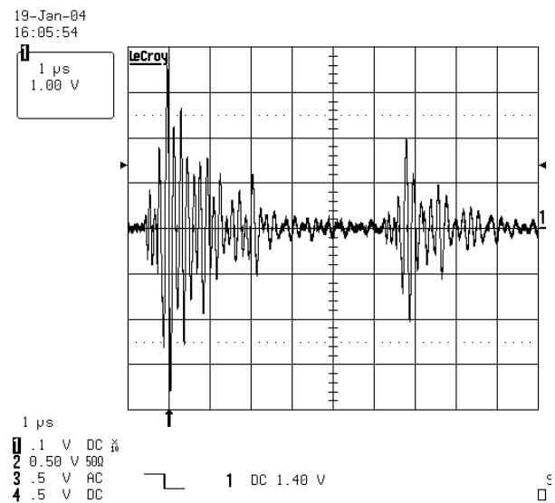
Figure 3. Voltage between the tip of a tool and ground. Peak voltage is ~3.6V
